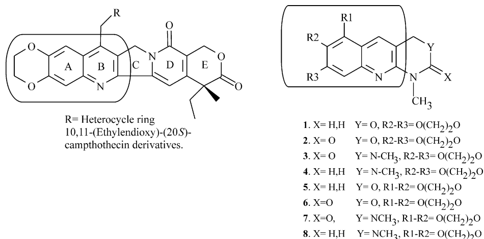
Figure 1. Analogue compounds of camptothecin.
