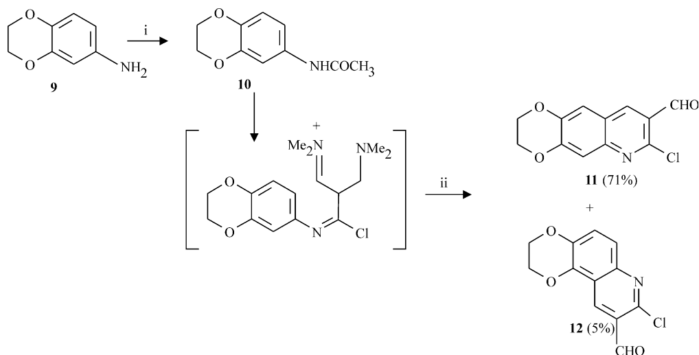
Scheme 1. Reagents and conditions: i (\text{CH}_3\text{CO})_2\text{O} , 140^\circ\text{C} ; ii \text{POCl}_3 /DMF, 90^\circ\text{C} .
